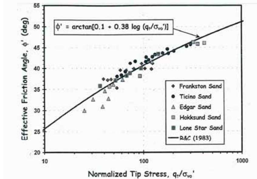
Figure 5-16 Relationship Between Friction Angle and the Effective Tip Resistance from CPTU Data
