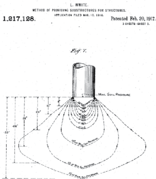
Assumed Stress Bulb Under Pile Tip Figure 6-3
