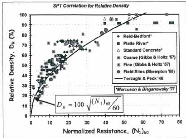
Figure 5-13 Relative Density of Clean Sands from Standard Penetration Test Data
