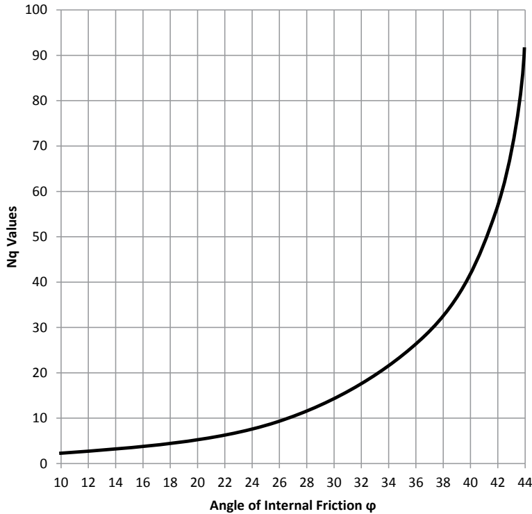
Bearing Capacity Factor N_q vs Soil Friction Angle \phi Figure 8-12
